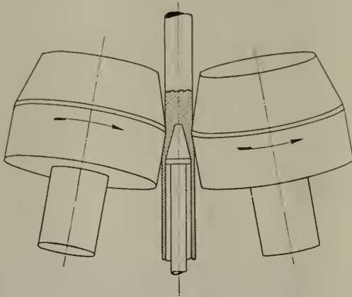
DIAGRAM OF PIERCING OPERATION
